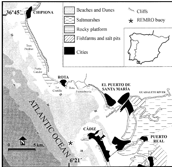
Fig. 1. Location map and main morphological characteristics of the studied littoral.
