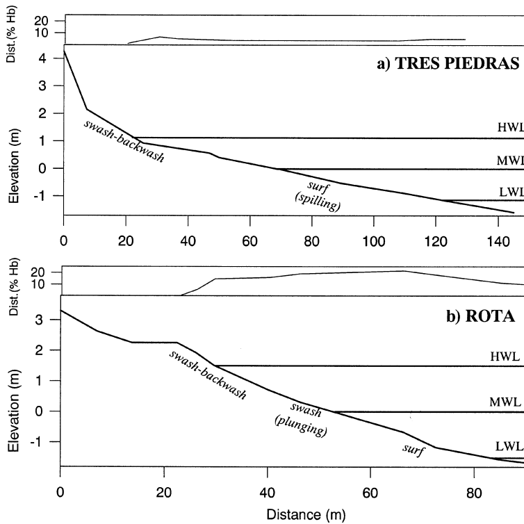
Fig. 8. Cross-shore variability of average disturbance depth in the two main morphodynamic classes: (a) dissipative, Tres Piedras beach; (b) reflective, Rota beach.
