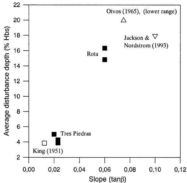
Fig. 9. Relation between average disturbance depth (percentage of breaking wave height) and beach gradient for the studied beaches (full symbols) and average values observed by other authors (empty symbols).
